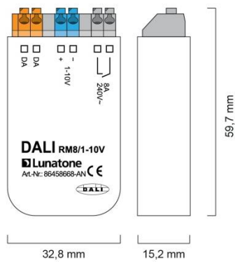
Geometrie RM8 PWM Geometrie RM8 1-10V
