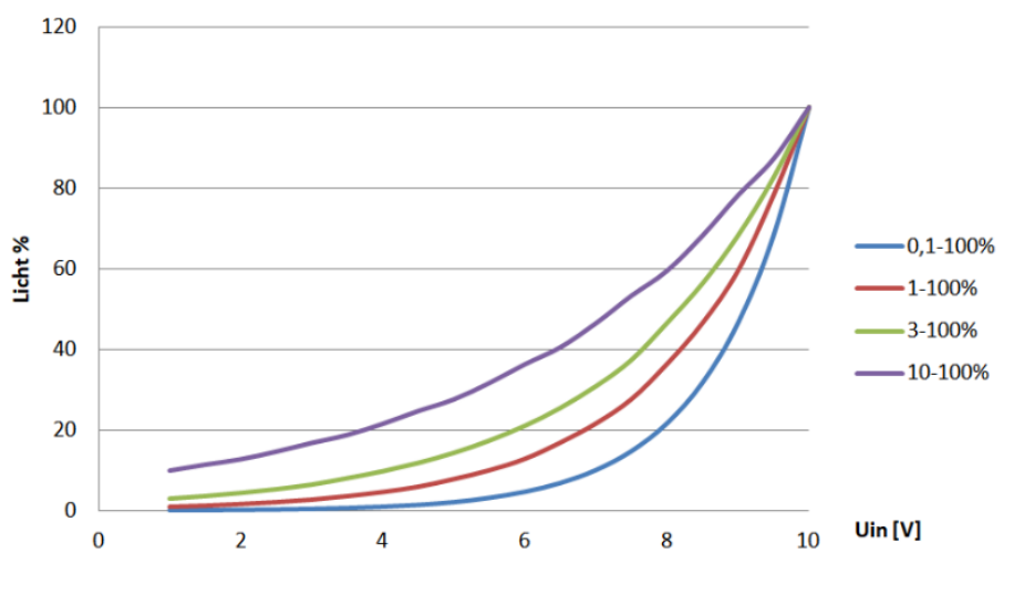
Light level of a DALI-ballast connected to the converter (corresponding to IEC62386-102). The light values in% are to be seen in connection with a DALI control gear.
