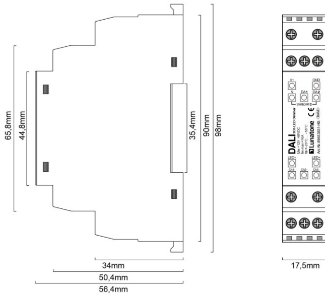
dimensions DIN rail housing Version 16A Art.Nr.: 89453831-HS
