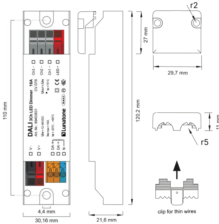
dimensions remote ceiling Version 16A Art.Nr.: 89453831 Version 10A Art.Nr.: 86459571
