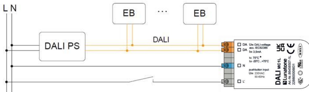
wiring diagram
