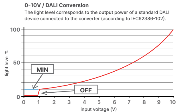
V4: Dimming: 10-100% <1V: MIN (10%) (blue curve)
