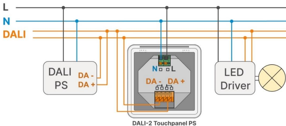
Figure 4 installation example DALI-2 Touchpanel PS with an additional DALI PS on the DALI bus
