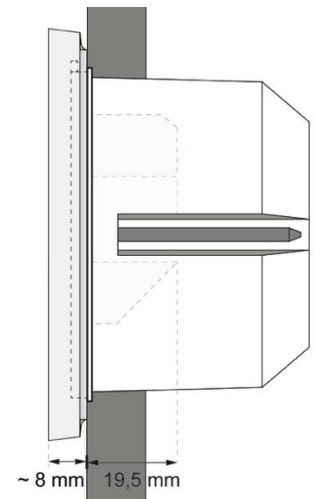
installed Touchpanel
