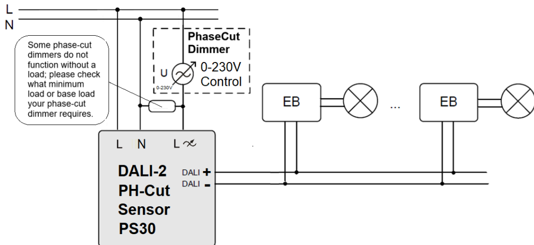
typical application DALI-2 Phase Cut Sensor PS30
