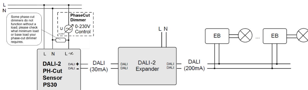
Control of 64 DALI-luminaires with a DALI-2 Phase Cut Sensor PS30 and the help of a DALI-2 Expander (ArtNr: 89452937)
