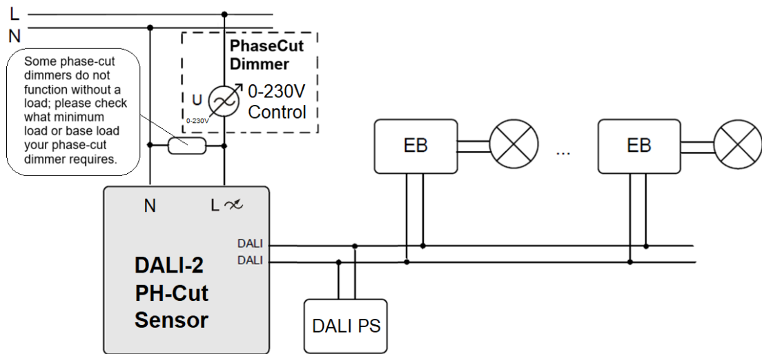
typical application DALI-2 Phase Cut Sensor
