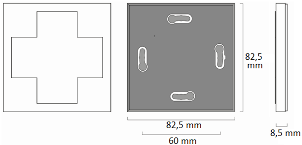
Geometrie wDALI-2 BT5 Switch Cross
