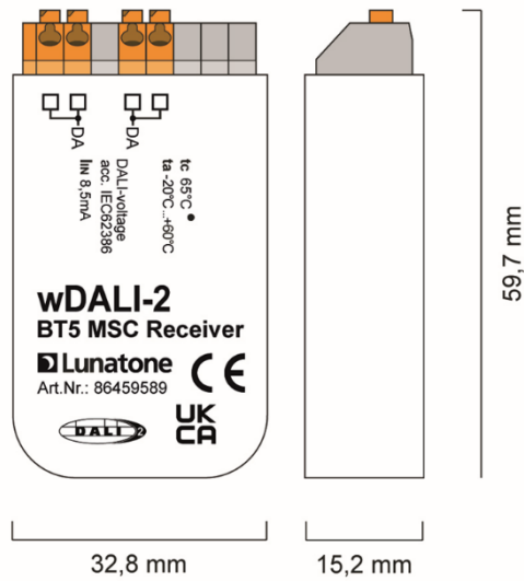
Geometrie wDALI-2 BT5 MSC Receiver
