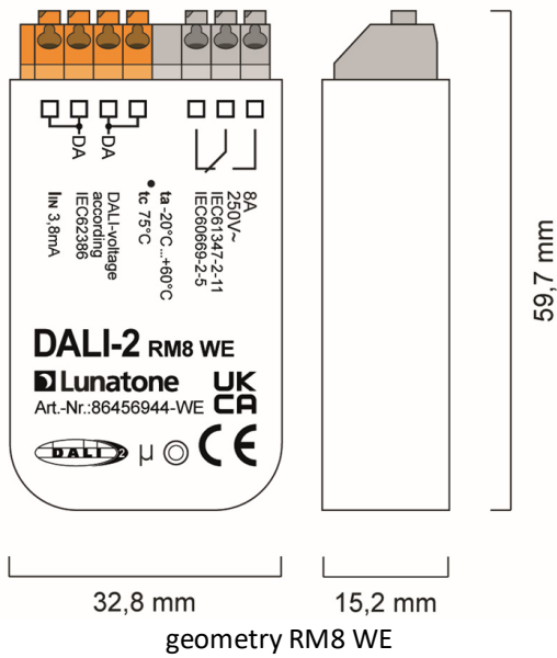
geometry RM8
