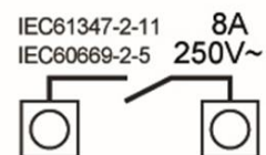
connection plan RM8 HS
